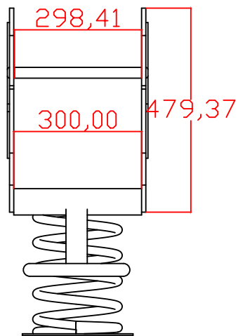
Vista Frontal
