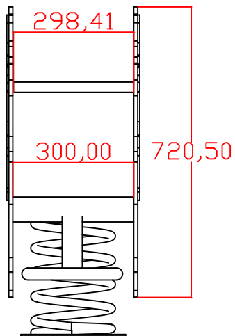
Vista Frontal
